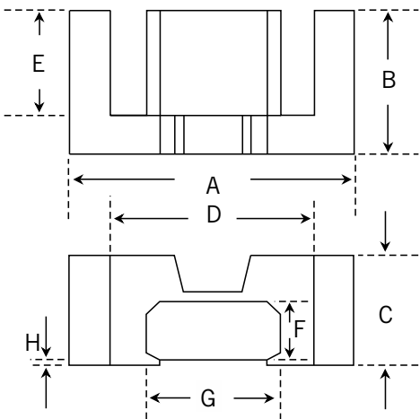
EFD CORE
