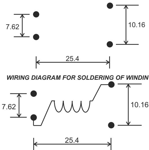
PCB DRILLING DETAIL (NOTE ALL DIMENSIONS mm)
