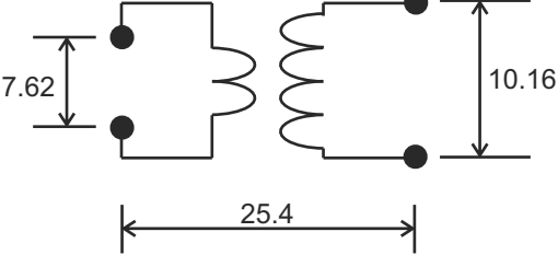
WIRING DIAGRAM FOR SOLDERING OF WINDINGS
