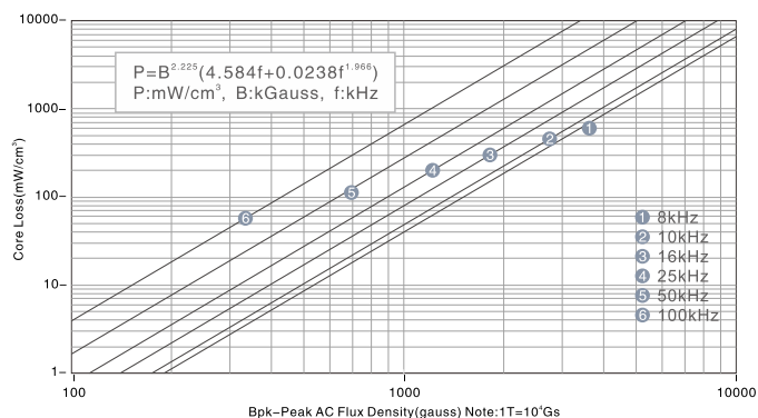
Typical Core Loss Curves (60μ, 75μ, 90μ, 125μ)
