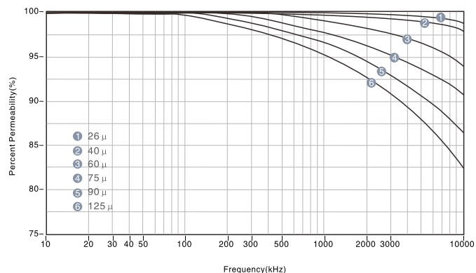
Permeability vs. Frequency
