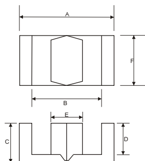
EED CORE
