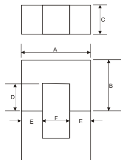
U CORE
